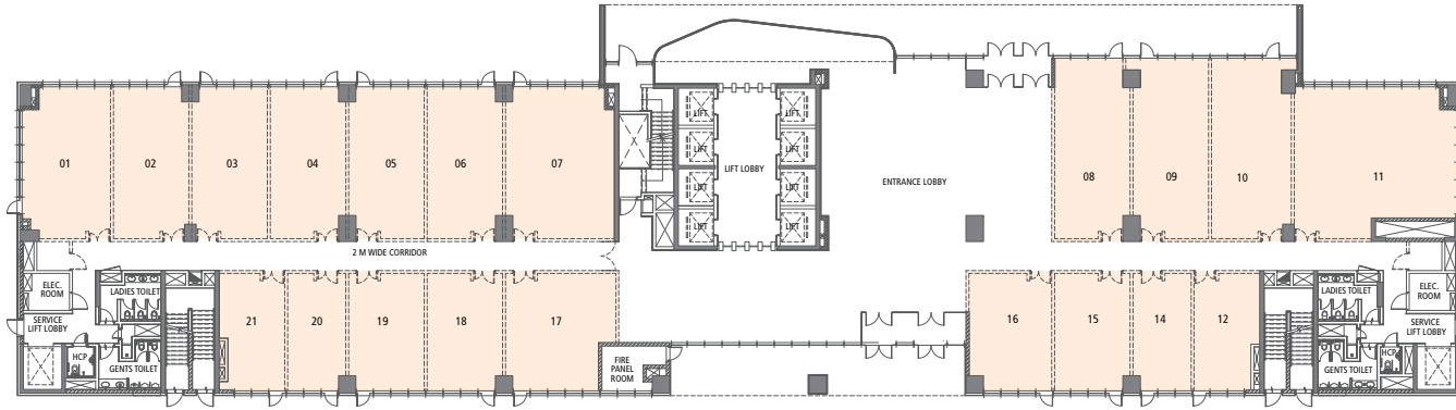
Tower B Ground Floor Plan - 21,712 sq. ft.
